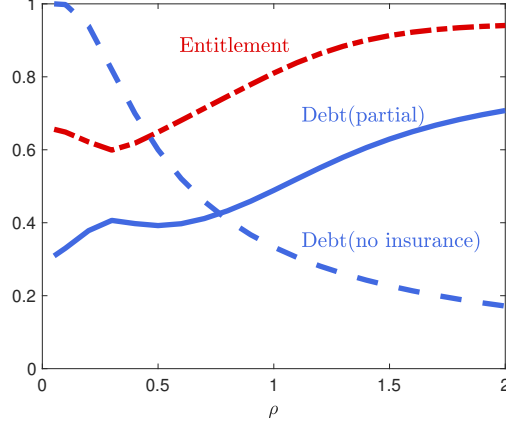
Figure 4: Debt and entitlements ( c_{A,1} ) in the partial insurance model against the value of \rho . The allocations are the solution for the numerical problem that considers u(c, g) = \frac{c^{1-\rho}-1}{1-\rho} + \frac{g^{1-\rho}-1}{1-\rho} , with y = 1 , \beta = 1 , \bar{g} = 0.05 , and c_{B,0} = 0.165 .
