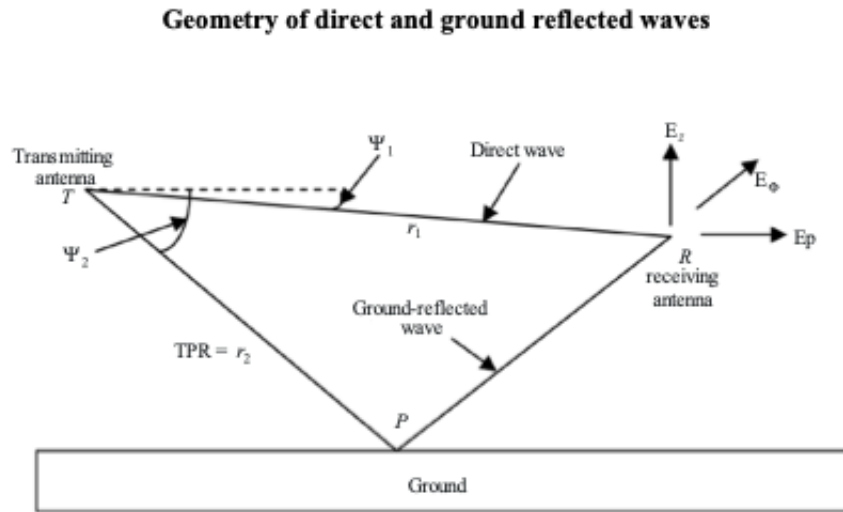
Figure B.6: Propagation of the Space Wave Component of the Ground Wave
