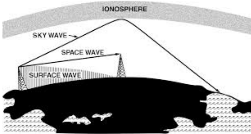
Figure B.5: Sky Waves Versus Ground Waves
