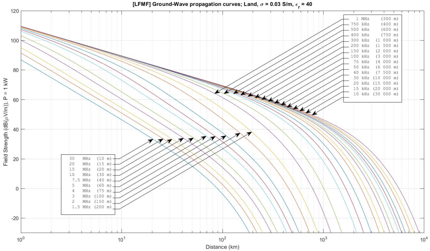
Figure B.9: ITU LFMF Propagation Curves, \sigma = .03S/m , \epsilon = 40
