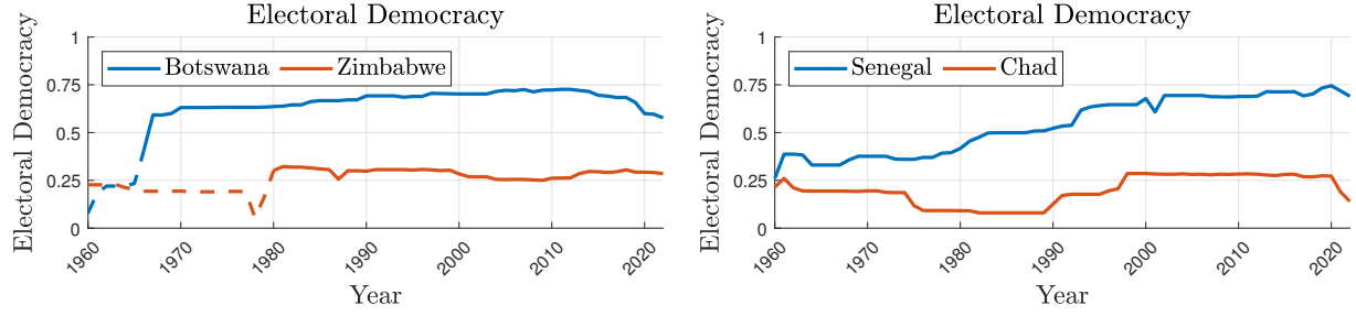
Figure 7: Post-Colonial Rule. Each panel depicts Electoral Democracy Index from V-Dem (Coppedge et al., 2023). Dashed line indicates colonial periods.
