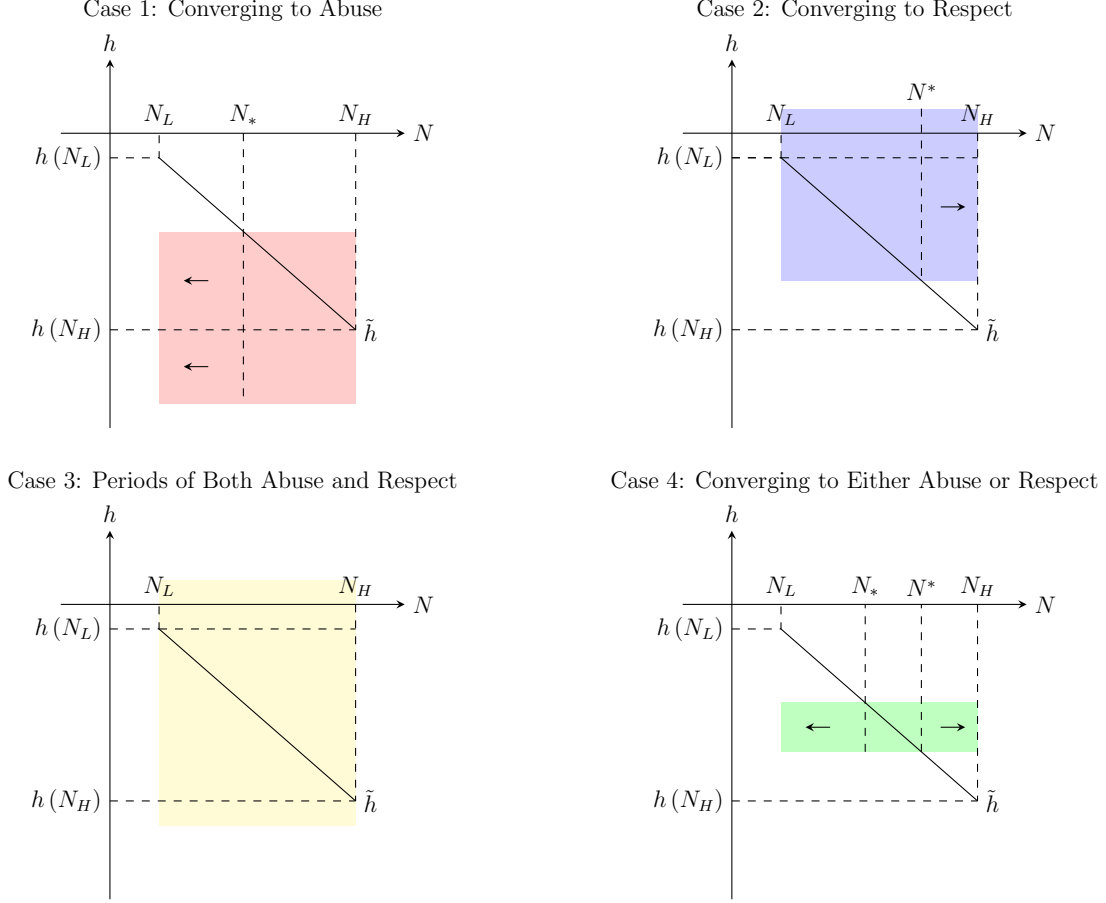
Figure 1: Theorem 2. The top left panel depicts Case 1; the top right panel Case 2; the bottom left panel Case 3; and the bottom right panel Case 4.
