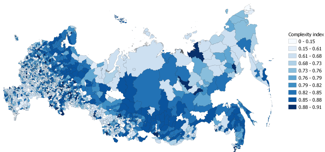
Figure 3: Complexity index
