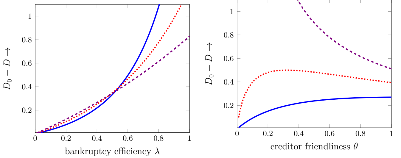
Figure 2: The plots above show how the equilibrium write-down D_0 - D depends on \lambda (left panel) and \theta (right panel) with D_0 endogenous. The parameters used are as follows: both panels: F(v) = v/100 and I = 10 ; left panel: \theta = 0.4 (solid blue), 0.6 (dotted red), 0.8 (dashed violet); right panel: \lambda = 0.4 (solid blue), 0.6 (dotted red), 0.8 (dashed violet).
