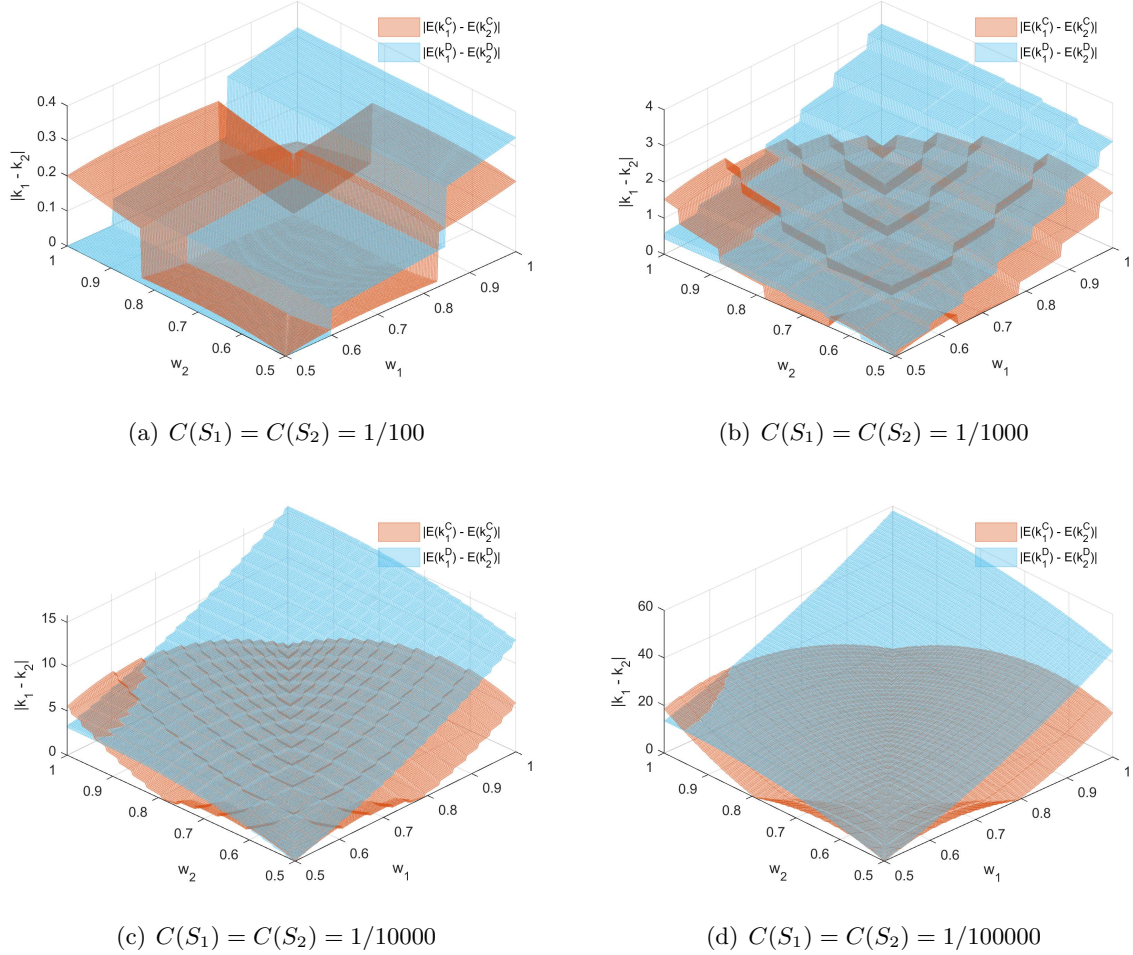
Figure 5: Comparison between |E(k_1^{\text{C}}) - E(k_2^{\text{C}})| and |E(k_1^{\text{D1}}) - E(k_2^{\text{D1}})| .
