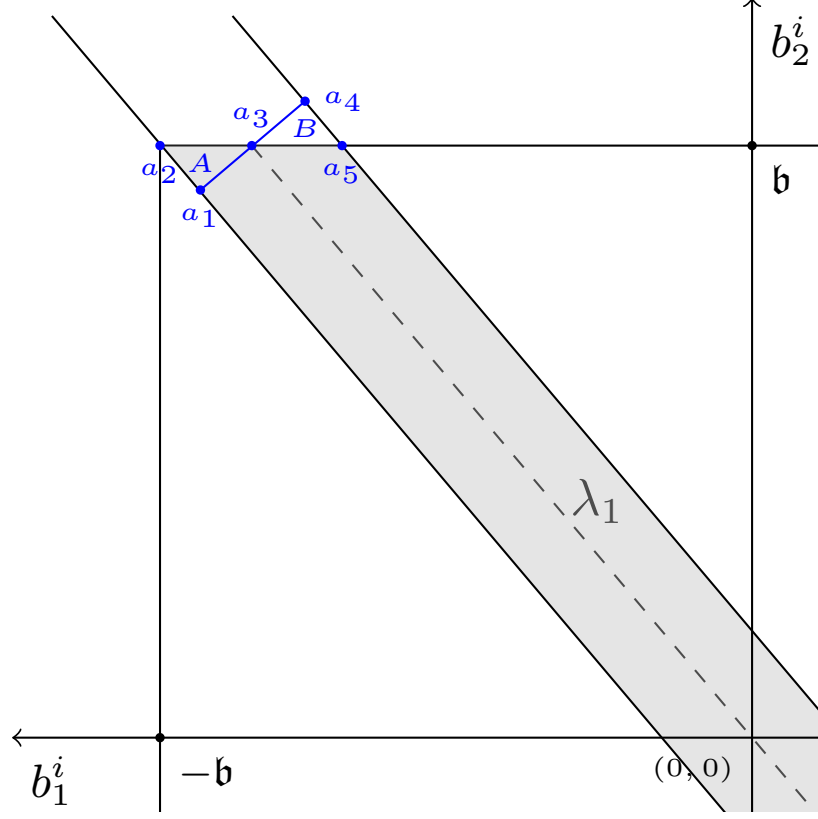
Figure 6: Probability of b \in \mathfrak{B}_1^c from the communication IC constraint
