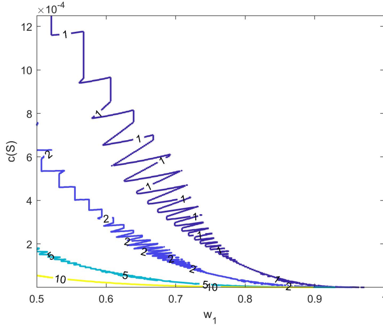
Figure 4: Contour for |E(k_1^C) - E(k_1^{D1})| for all w_1 and relevant C(S_1) .
