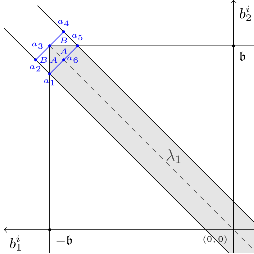
Figure 7: Probability of b \in \mathfrak{B}_1^c from the communication IC constraint
