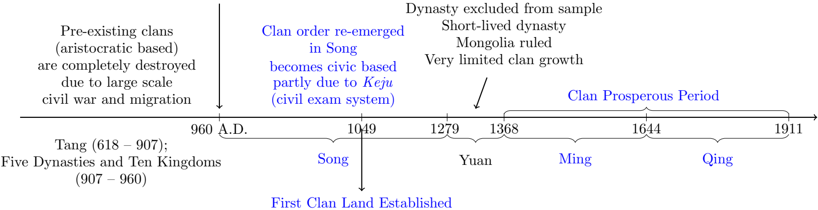
Figure 1: Timeline
