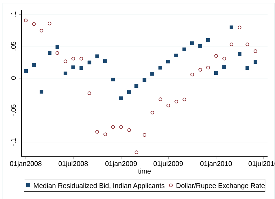
Figure 2: Median Residual Log Bids and Detrended Exchange Rates for India.
