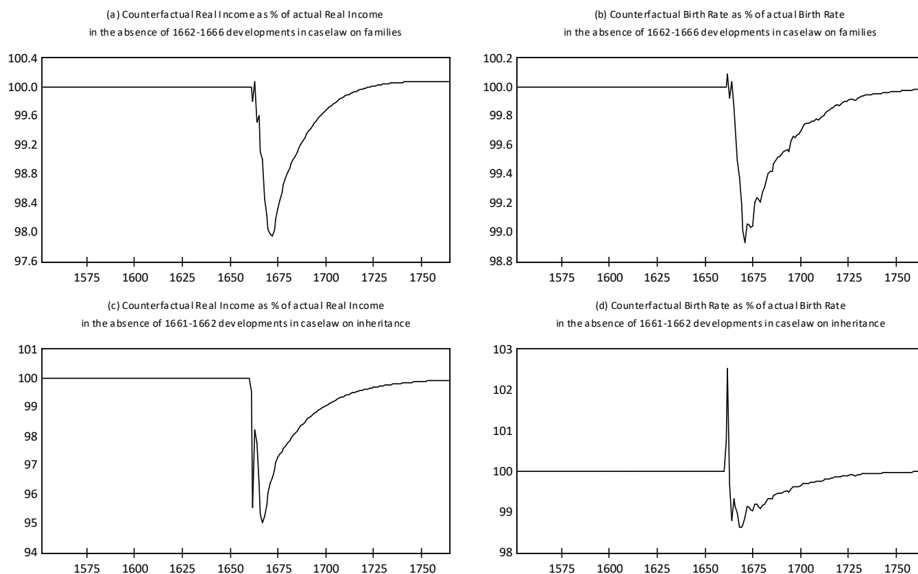
Figure 3: Counterfactual simulations
