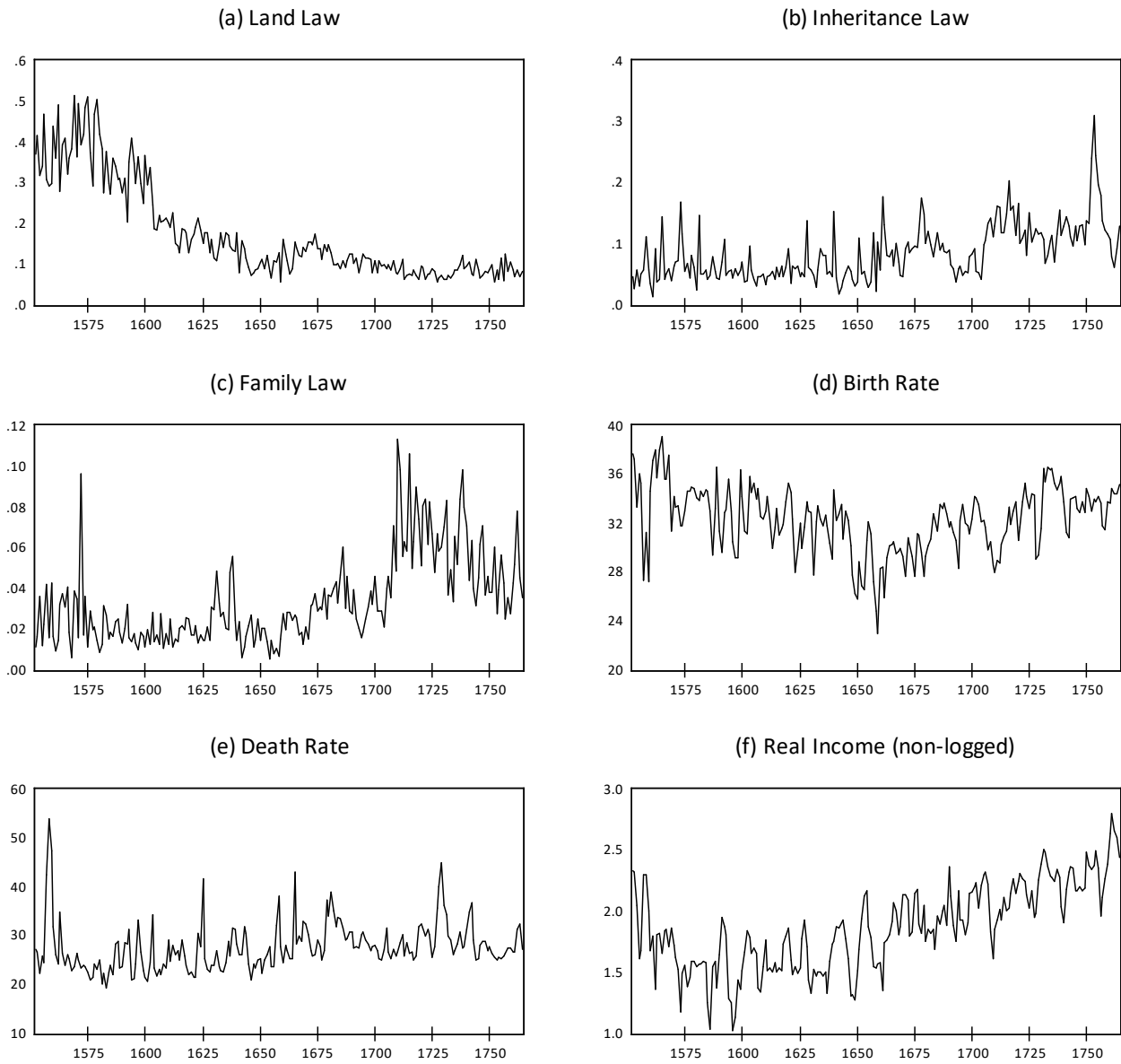
Figure 1: The time-series
