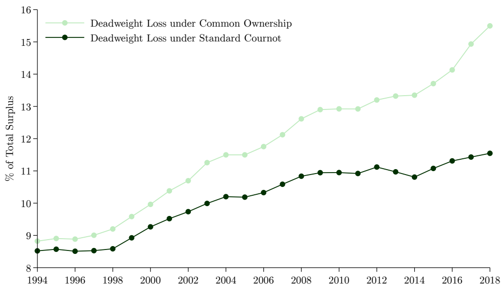
FIGURE NOTES: The figure plots the estimated deadweight loss (DWL) of oligopoly and of oligopoly and common ownership, between 1994 and 2018. The dark green line is the DWL of oligopoly, the % difference in total surplus between the Cournot equilibrium and the Perfect Competition scenario. The light green line is the % difference between the Cournot Common Ownership equilibrium and the Perfect Competition scenario.
