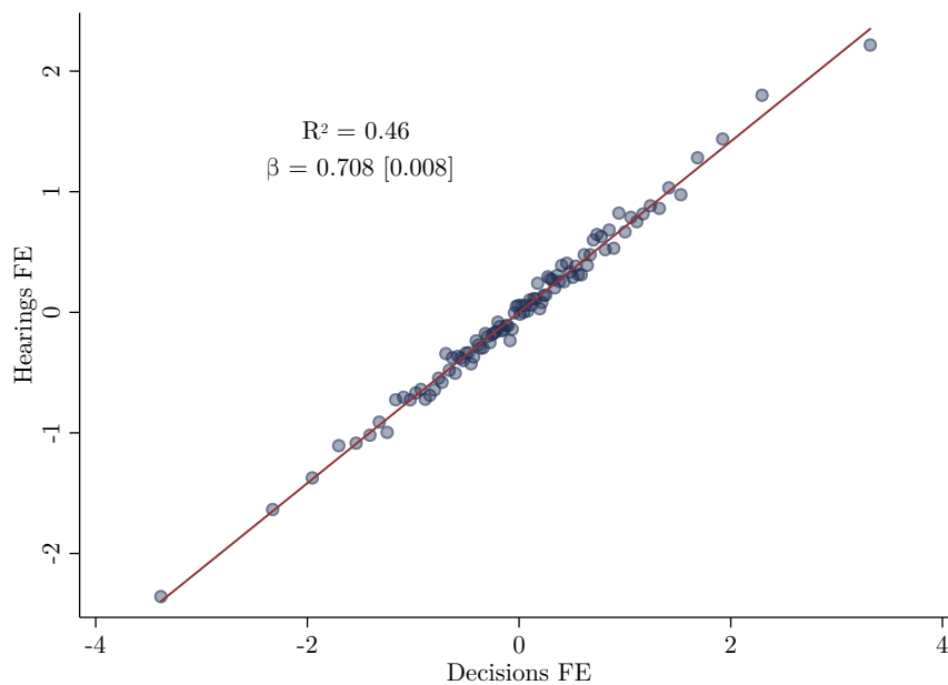
Figure 7: Binscatter of hearing and case disposition fixed-effects
