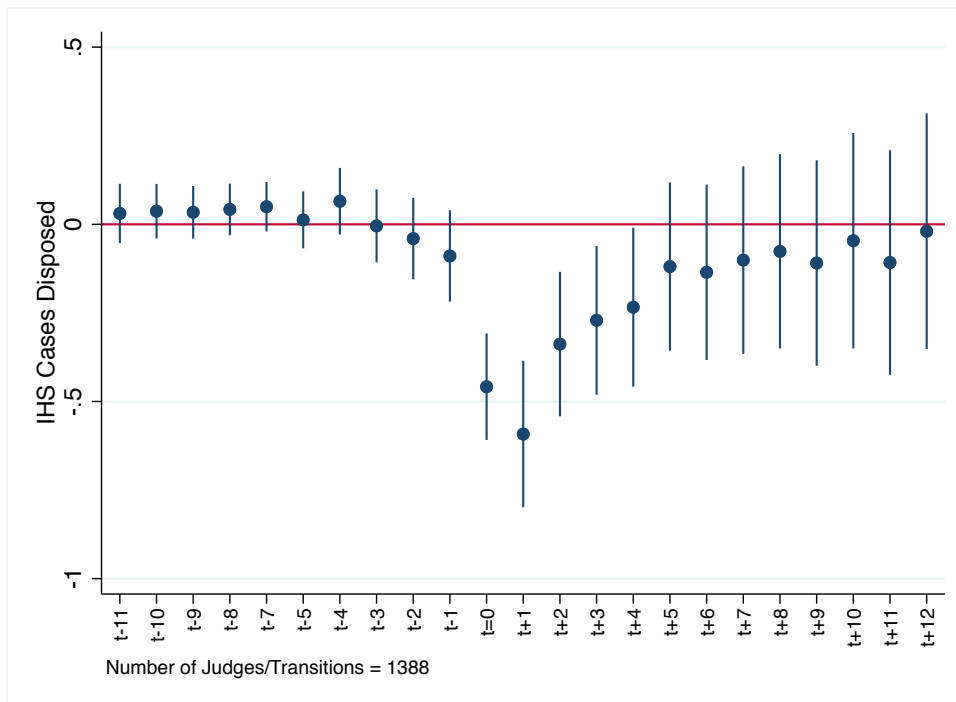
Figure 8: Event-study around judicial district movement
