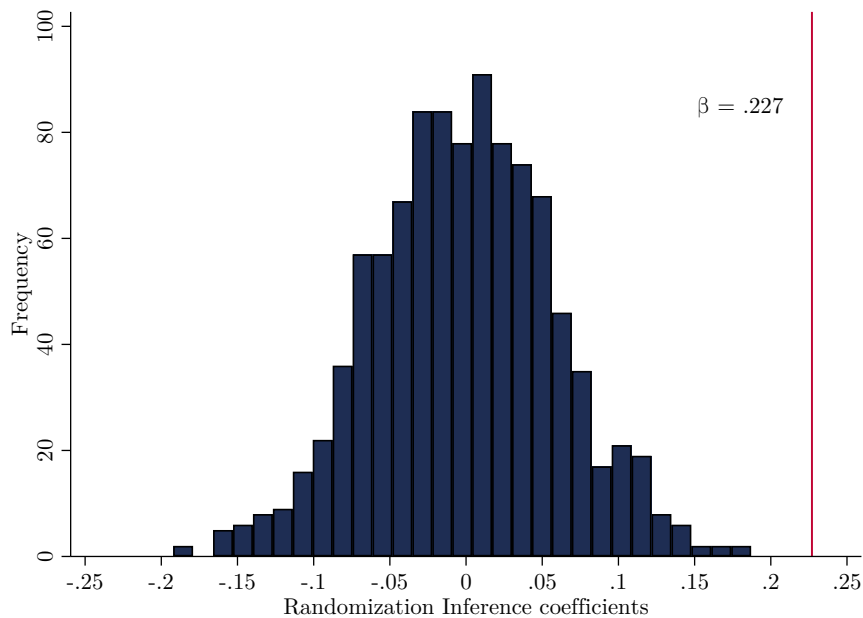
Figure 9: Histogram of simulated beta-coefficients
