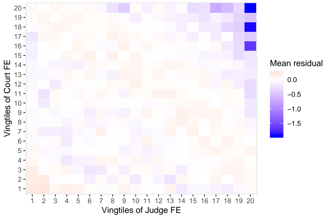
Figure 5: Actual heatmap estimated from the data
