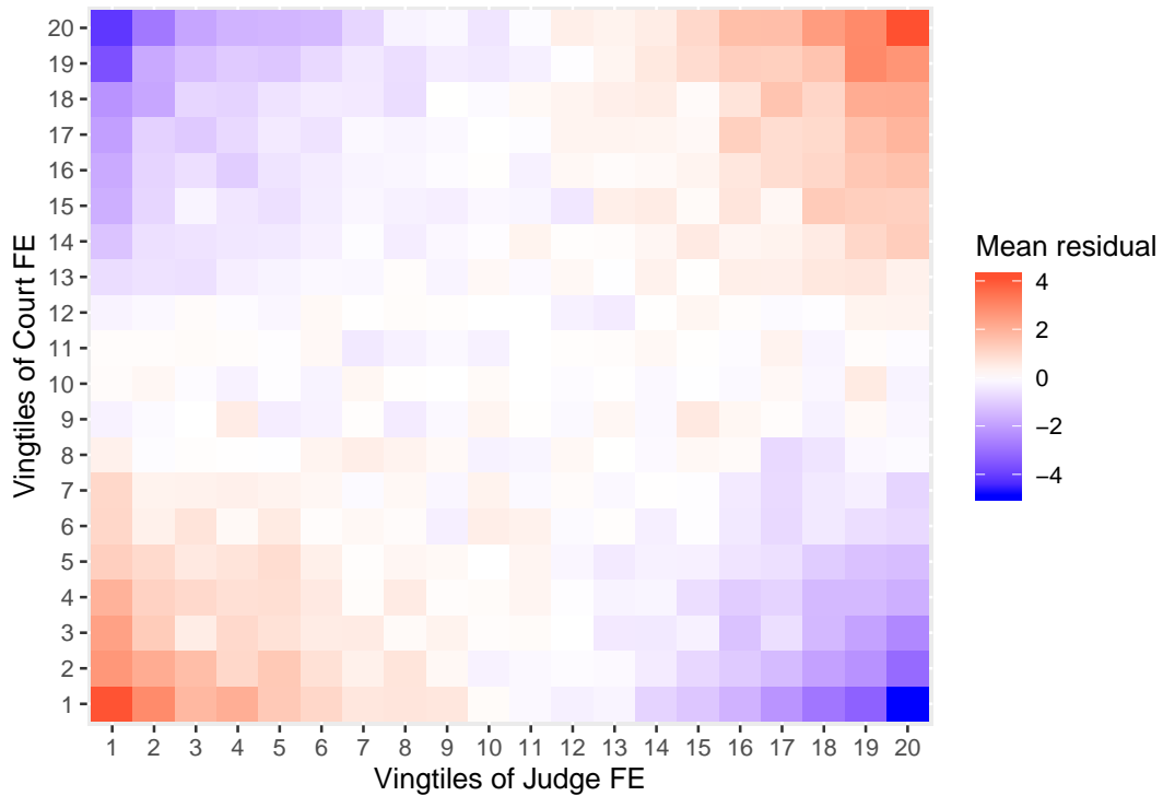
Figure 6: Simulated residuals of misspecified model
