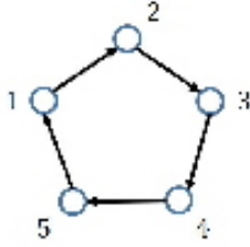
Figure 7: The cyclic network, for which there is no equilibrium for some open set of parameters.
