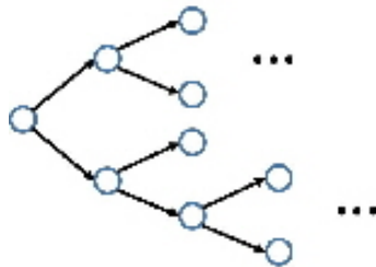
Figure 6: A binary tree network ( n = 2 ).
