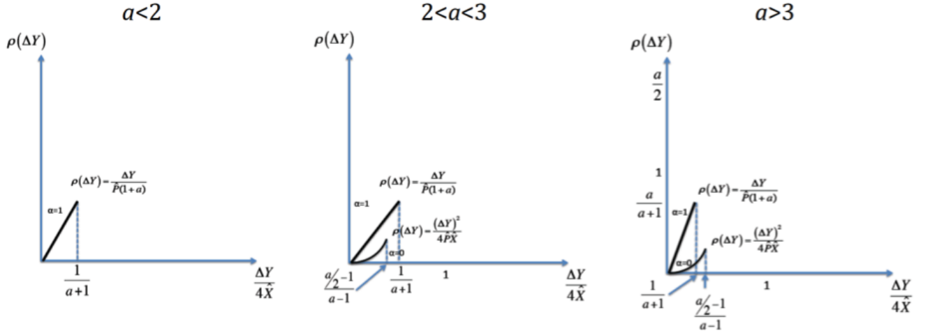
Figure 1: Equilibria.
