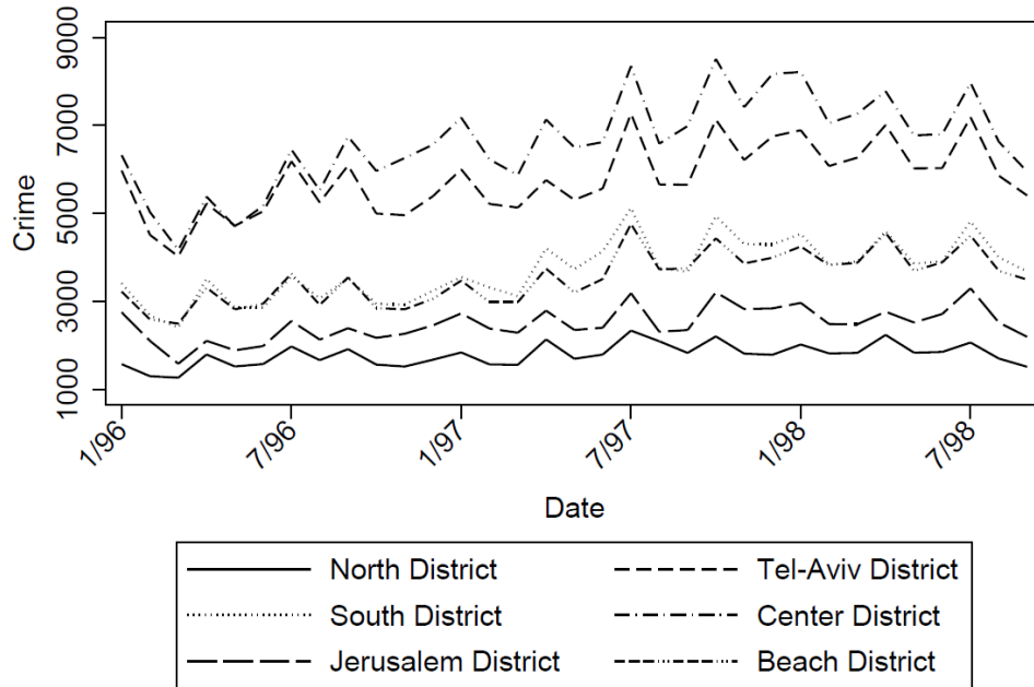
Figure 4: Pre-reform crime trends, by region
